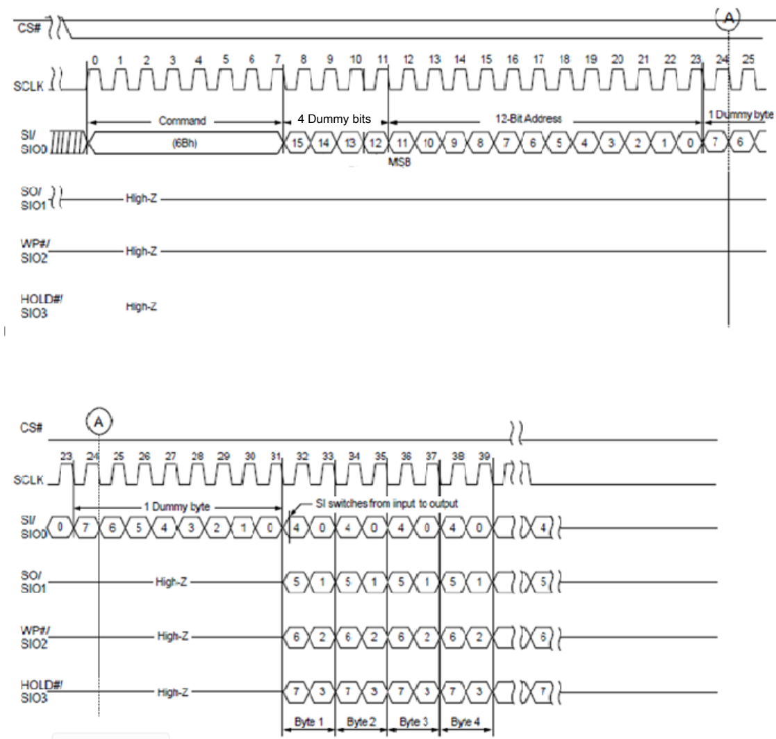
Figure 3.8 Read From Cache x4
