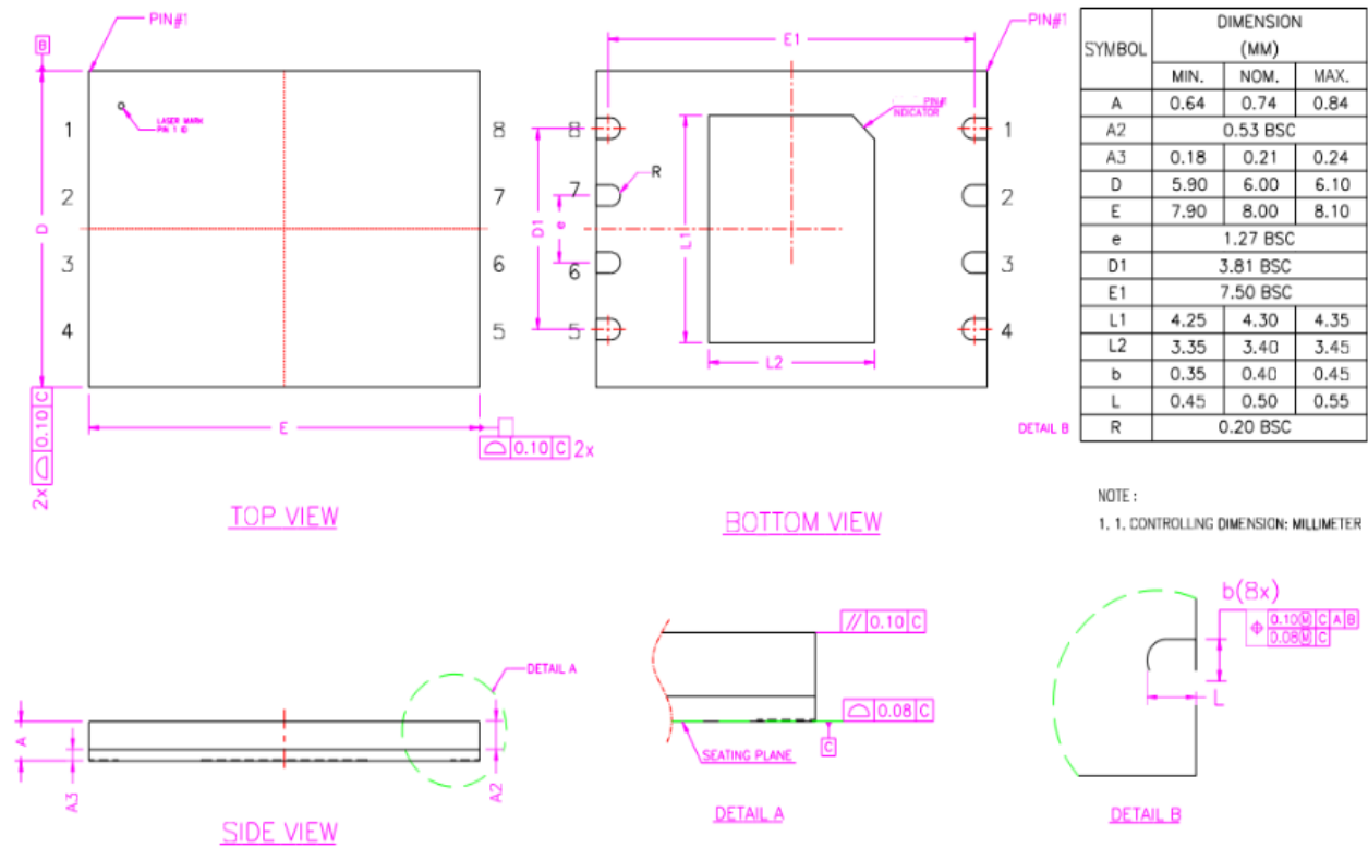
Figure 6.2 LGA (8*6mm)
